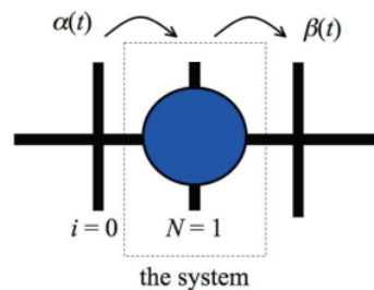
Fig. 2. The TASEP with a single site. The lattice system only consists of one site that is the site given in the dotted box. Site i = 0 is considered as the left reservoir and the site N + 1 acts as the right reservoir. The shaded (blue) circle is the particle occupying site N = 1
